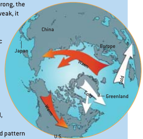
NORTH ATLANTIC OSCILLATION is depicted in its positive mode.
